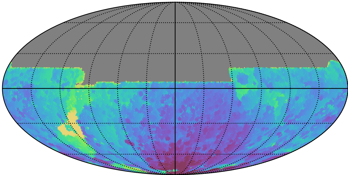
too_elab_heavy_r32_d2_griz_v3.4_10yrs All sky y band: Min HA
