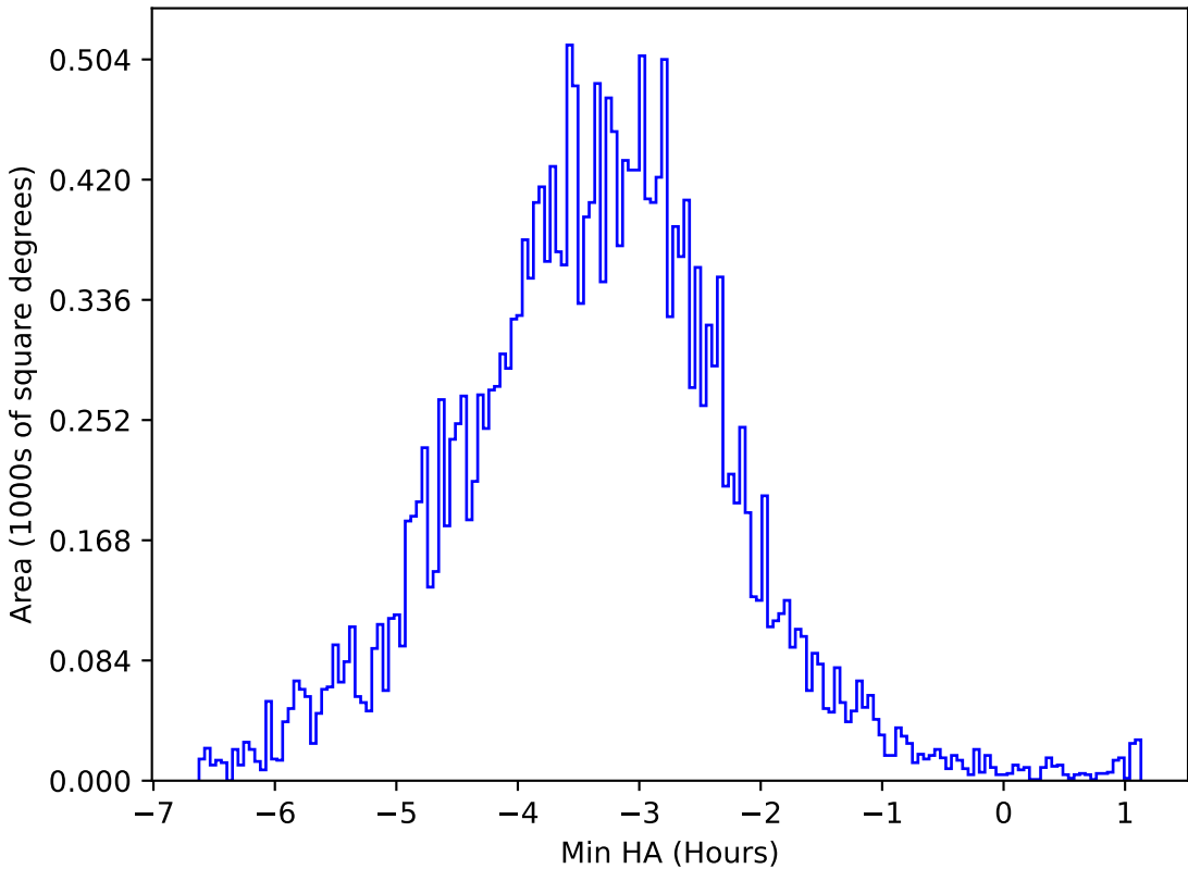
too_elab_heavy_r32_d2_griz_v3.4_10yrs All sky y band: Min HA
