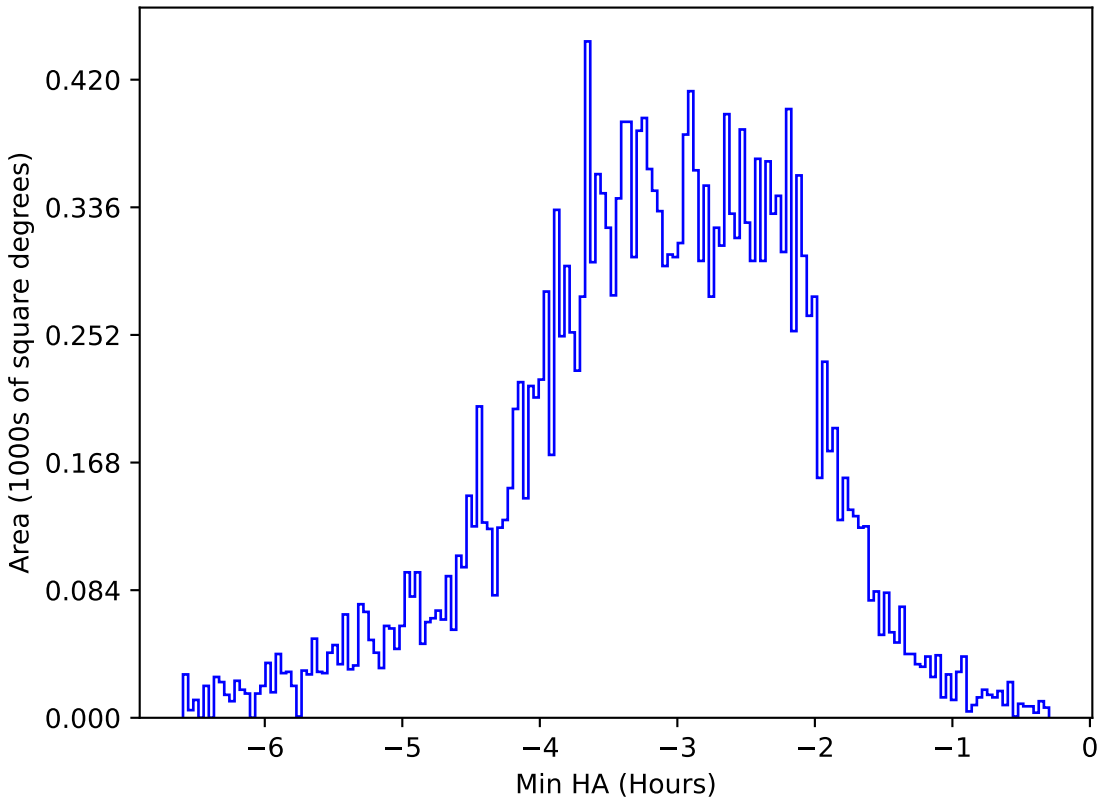
too_elab_heavy_r32_d2_griz_v3.4_10yrs All sky u band: Min HA
