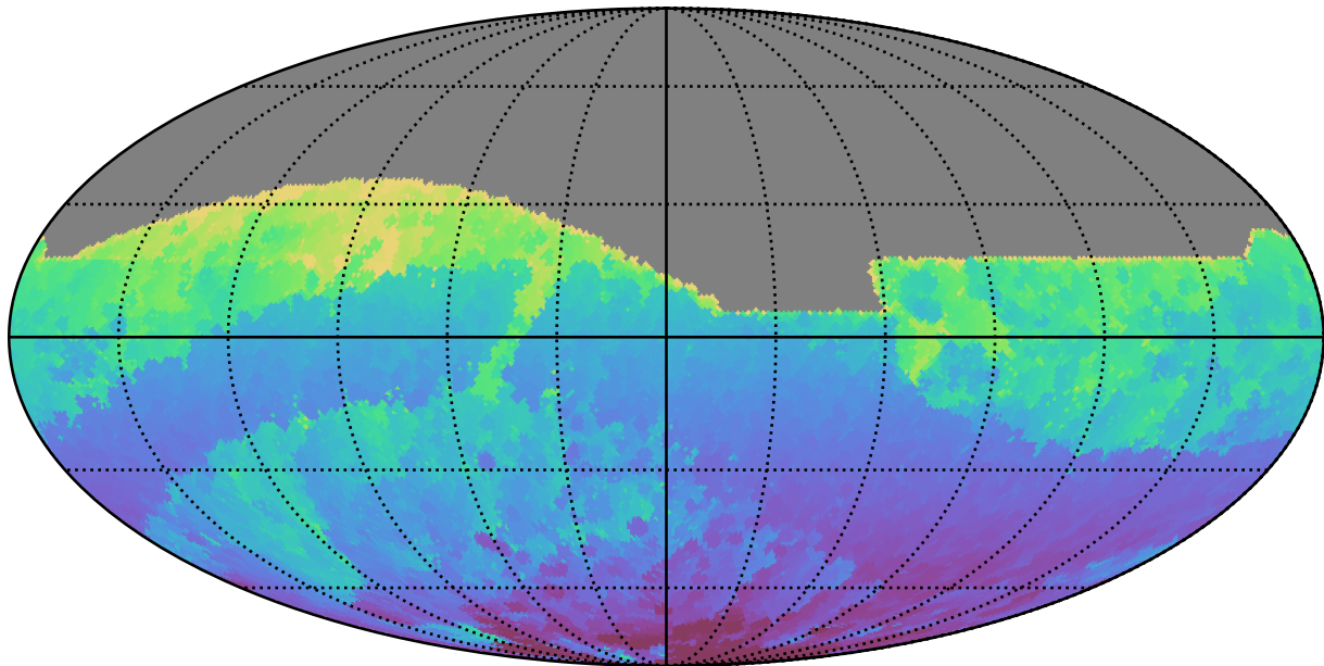
too_elab_heavy_r32_d2_griz_v3.4_10yrs All sky r band: Min HA
