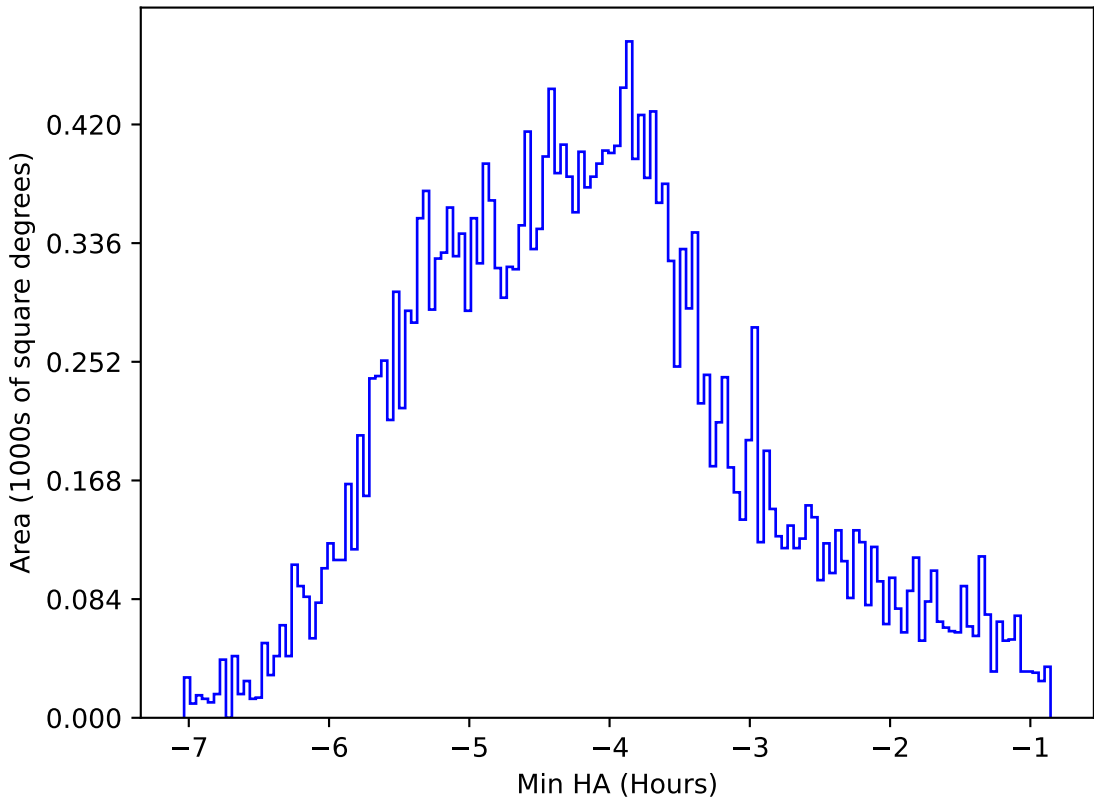
too_elab_heavy_r32_d2_griz_v3.4_10yrs All sky r band: Min HA
