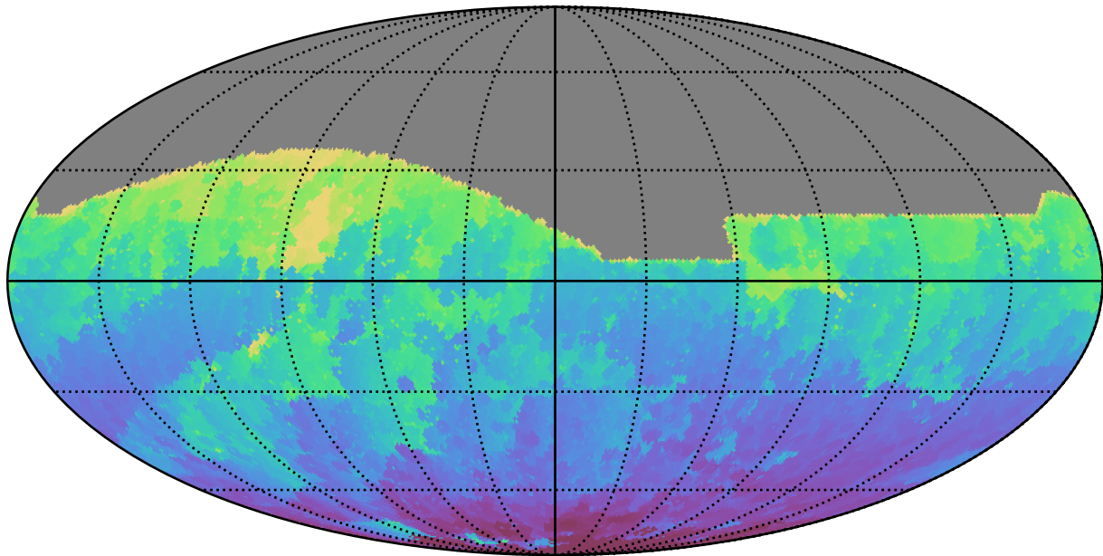
too_elab_heavy_r32_d2_griz_v3.4_10yrs All sky i band: Min HA
