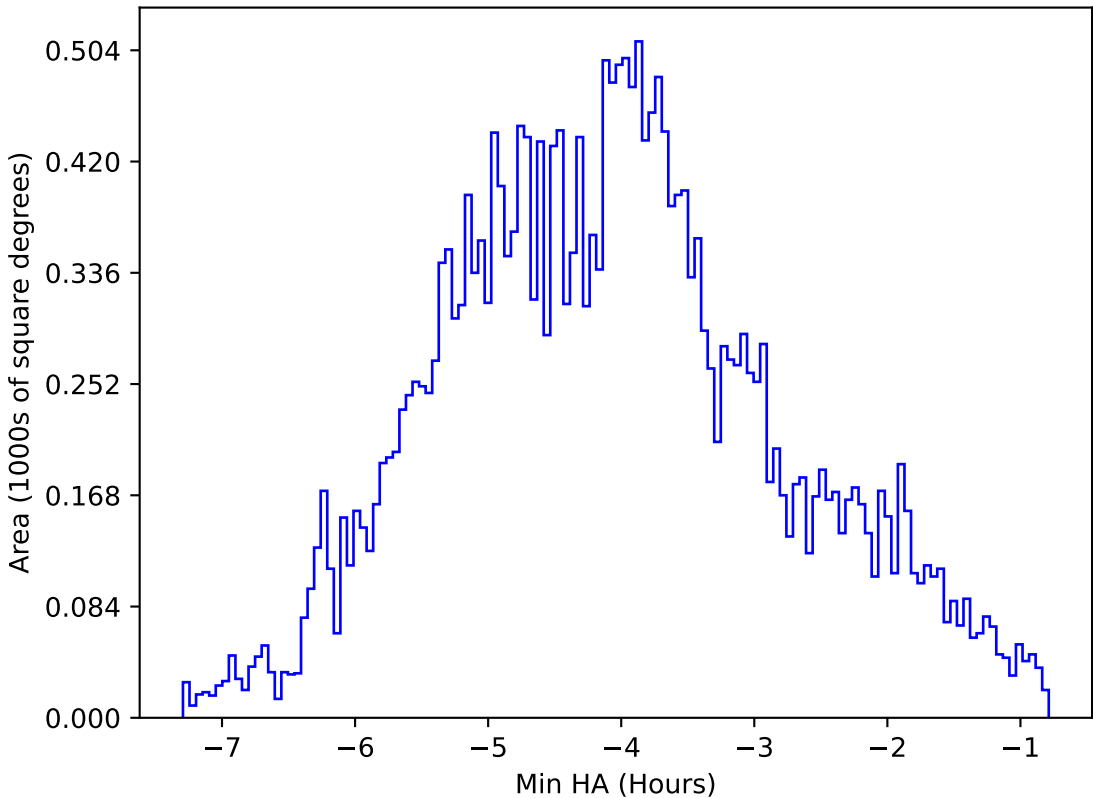
too_elab_heavy_r32_d2_griz_v3.4_10yrs All sky i band: Min HA
