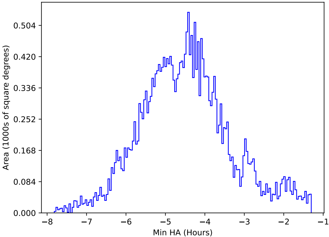
too_elab_heavy_r32_d2_griz_v3.4_10yrs All sky all bands: Min HA
