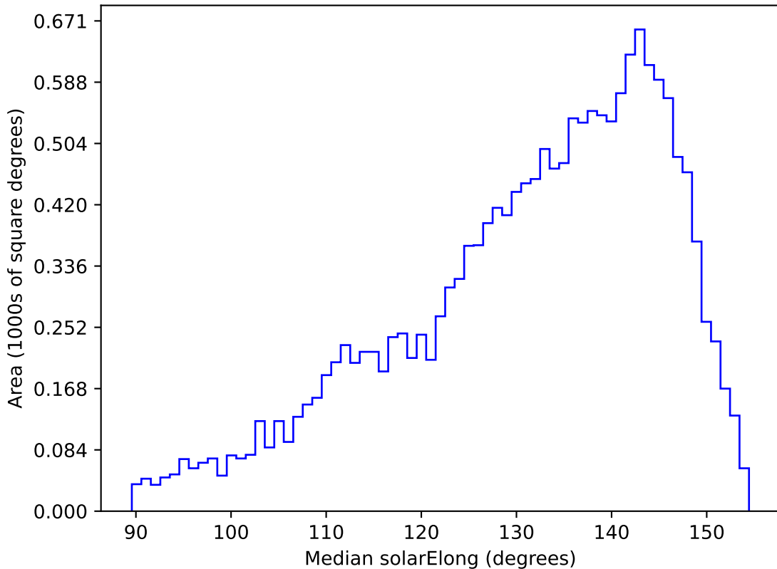
too_elab_heavy_r32_d2_griz_v3.4_10yrs WFD g band: Median solarElong
