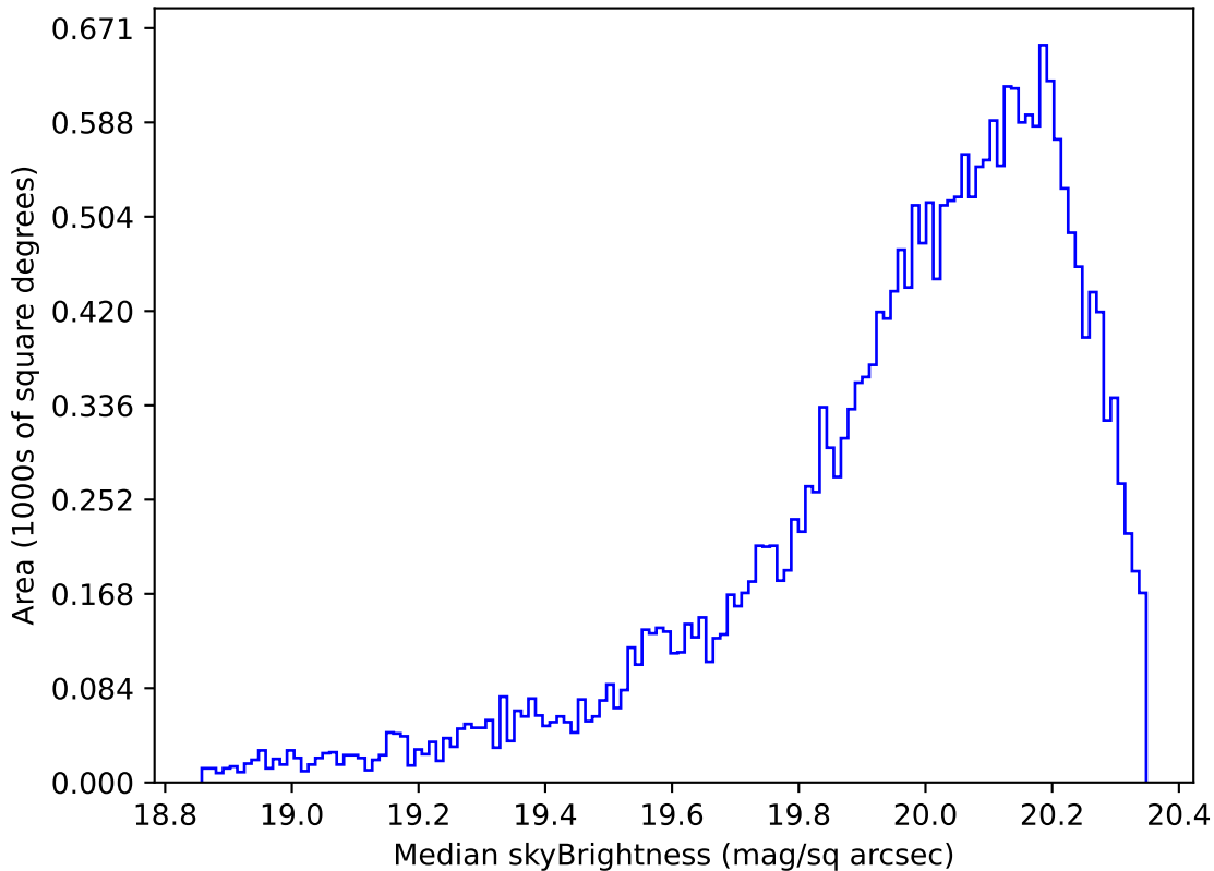
too_elab_heavy_r32_d2_griz_v3.4_10yrs Yr 1 i band: Median skyBrightness
