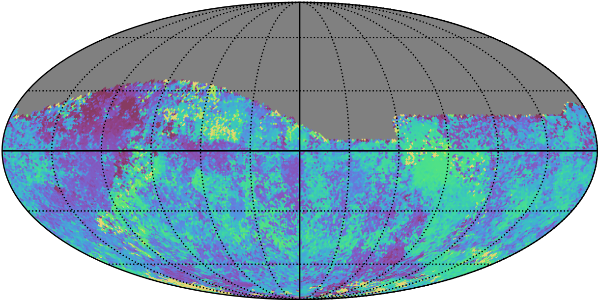
too_elab_heavy_r32_d2_griz_v3.4_10yrs Yr 1 all bands: Median skyBrightness
