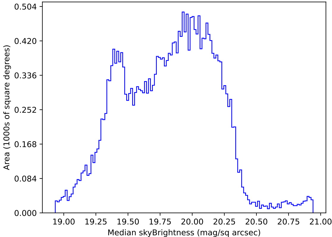
too_elab_heavy_r32_d2_griz_v3.4_10yrs Yr 1 all bands: Median skyBrightness
