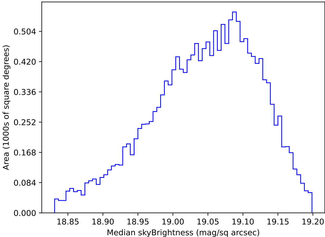
too_elab_heavy_r32_d2_griz_v3.4_10yrs WFD z band: Median skyBrightness
