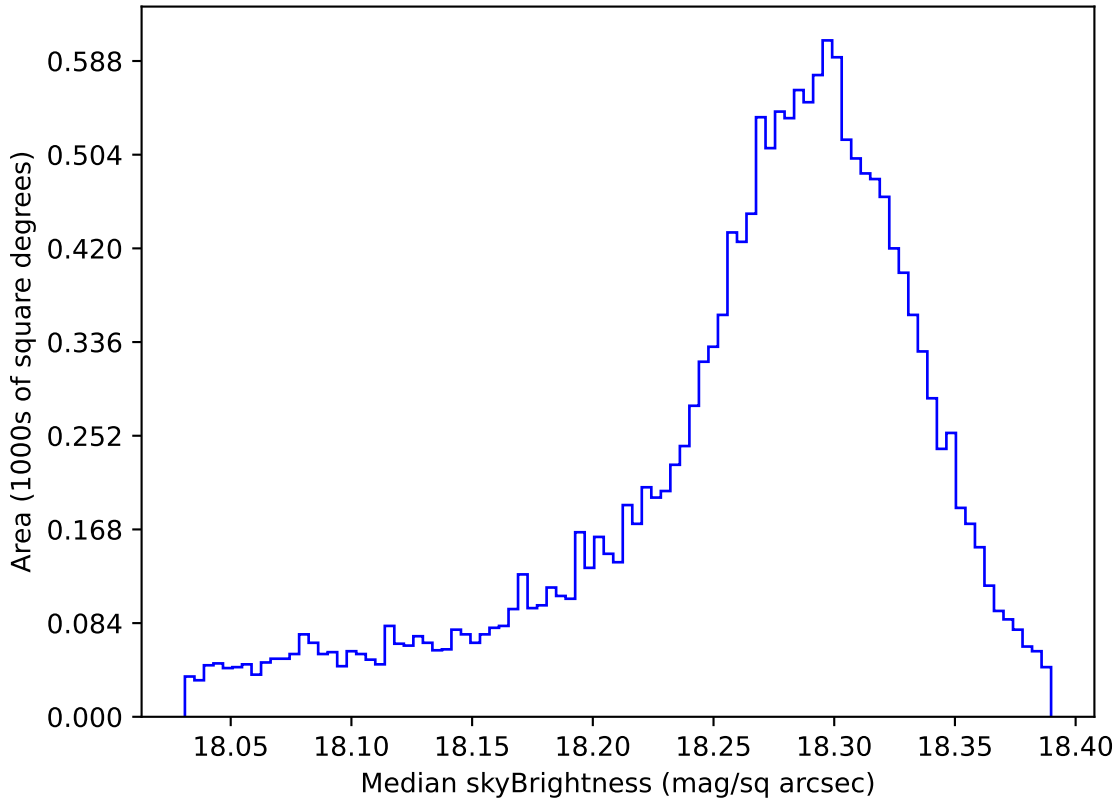
too_elab_heavy_r32_d2_griz_v3.4_10yrs WFD y band: Median skyBrightness
