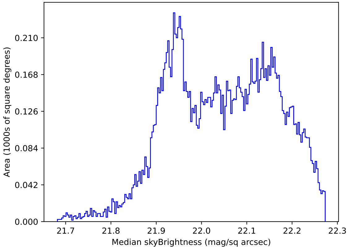
too_elab_heavy_r32_d2_griz_v3.4_10yrs WFD g band: Median skyBrightness
