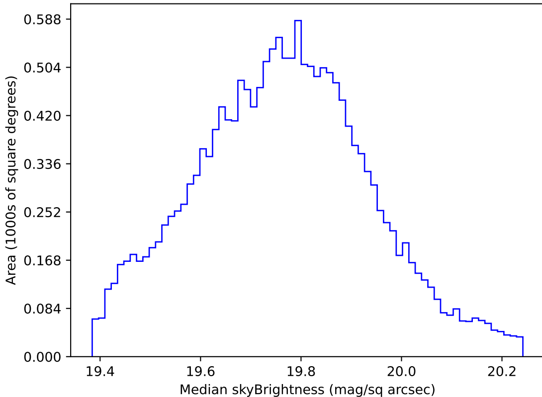
too_elab_heavy_r32_d2_griz_v3.4_10yrs WFD all bands: Median skyBrightness
