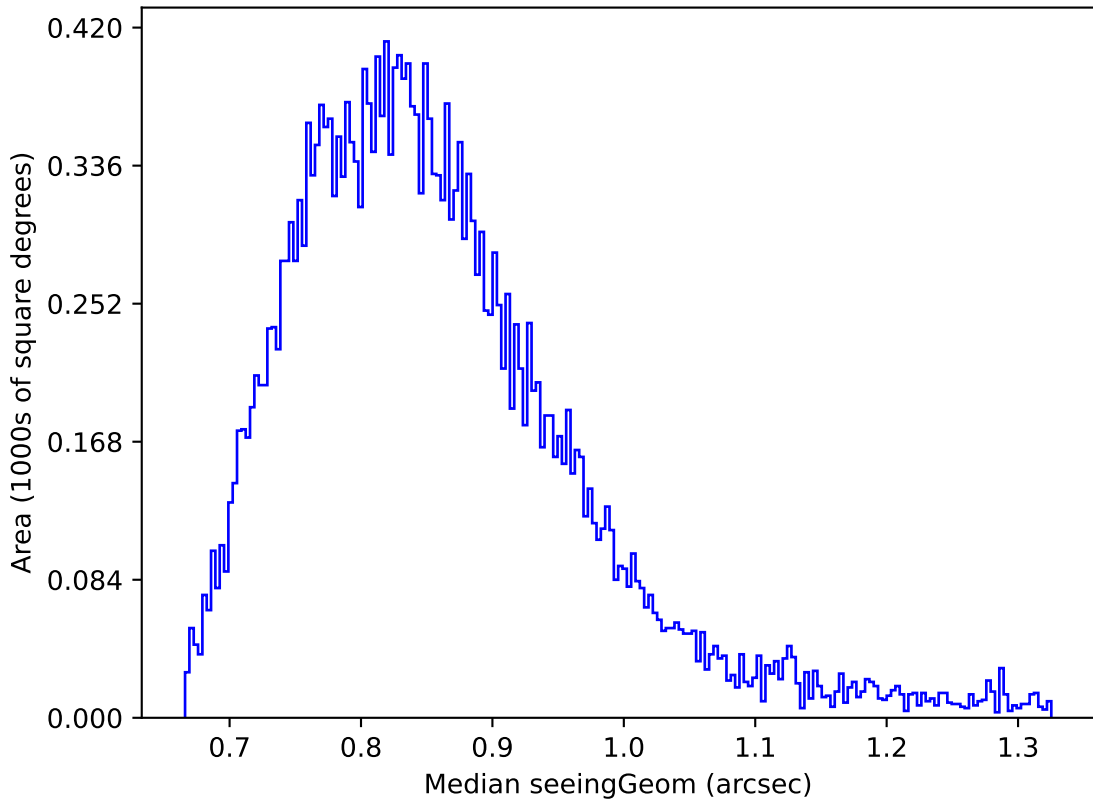
too_elab_heavy_r32_d2_griz_v3.4_10yrs Yr 1 z band: Median seeingGeom
