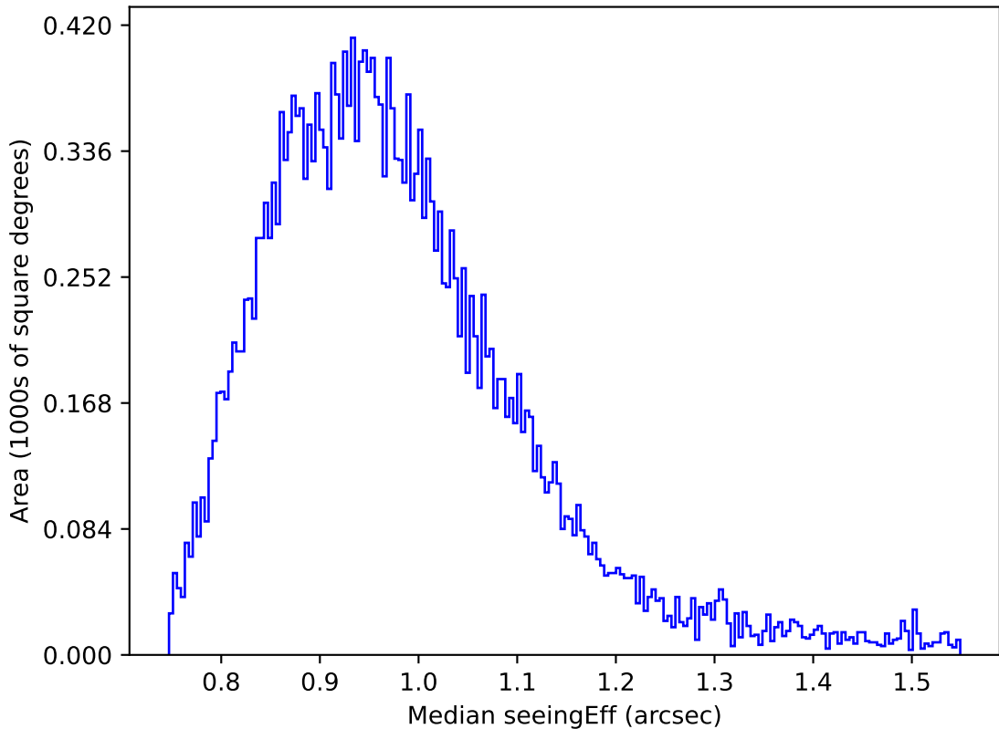
too_elab_heavy_r32_d2_griz_v3.4_10yrs Yr 1 z band: Median seeingEff
