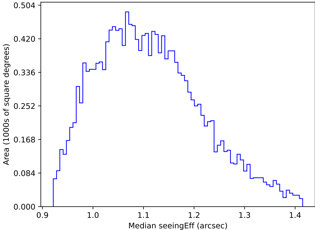
too_elab_heavy_r32_d2_griz_v3.4_10yrs WFD g band: Median seeingEff
