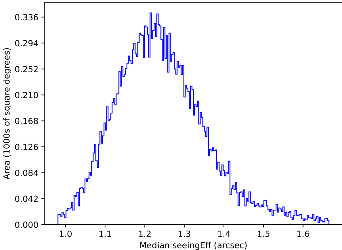
too_elab_heavy_r32_d2_griz_v3.4_10yrs All sky u band: Median seeingEff
