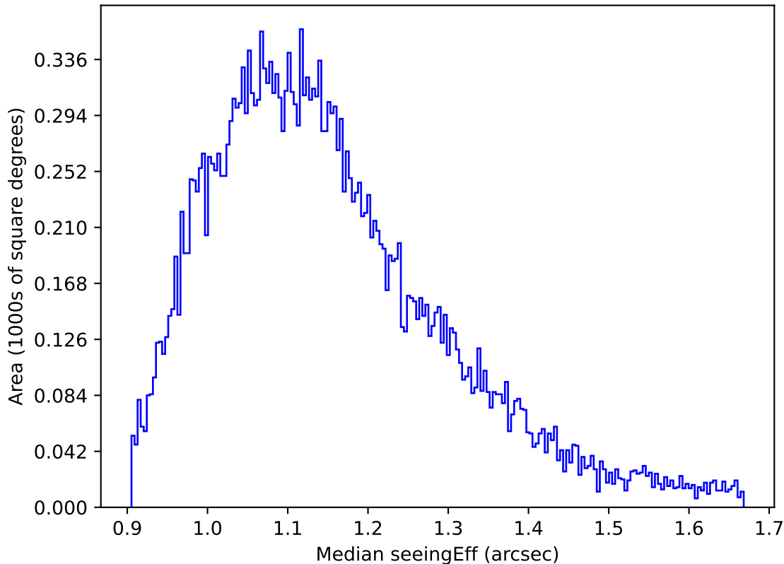
too_elab_heavy_r32_d2_griz_v3.4_10yrs All sky g band: Median seeingEff
