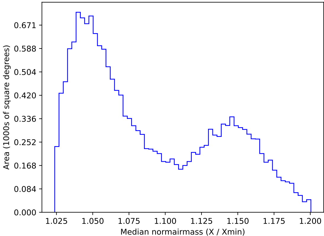
too_elab_heavy_r32_d2_griz_v3.4_10yrs WFD z band: Median normairmass
