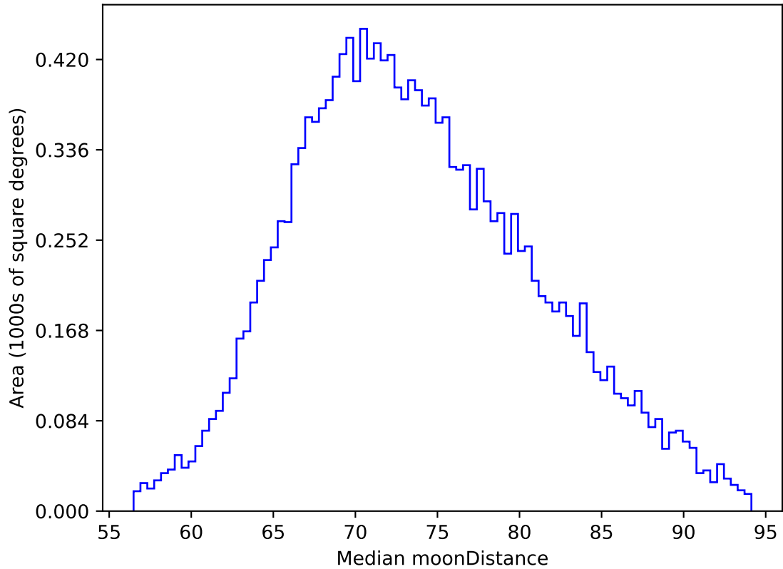
too_elab_heavy_r32_d2_griz_v3.4_10yrs WFD z band: Median moonDistance
