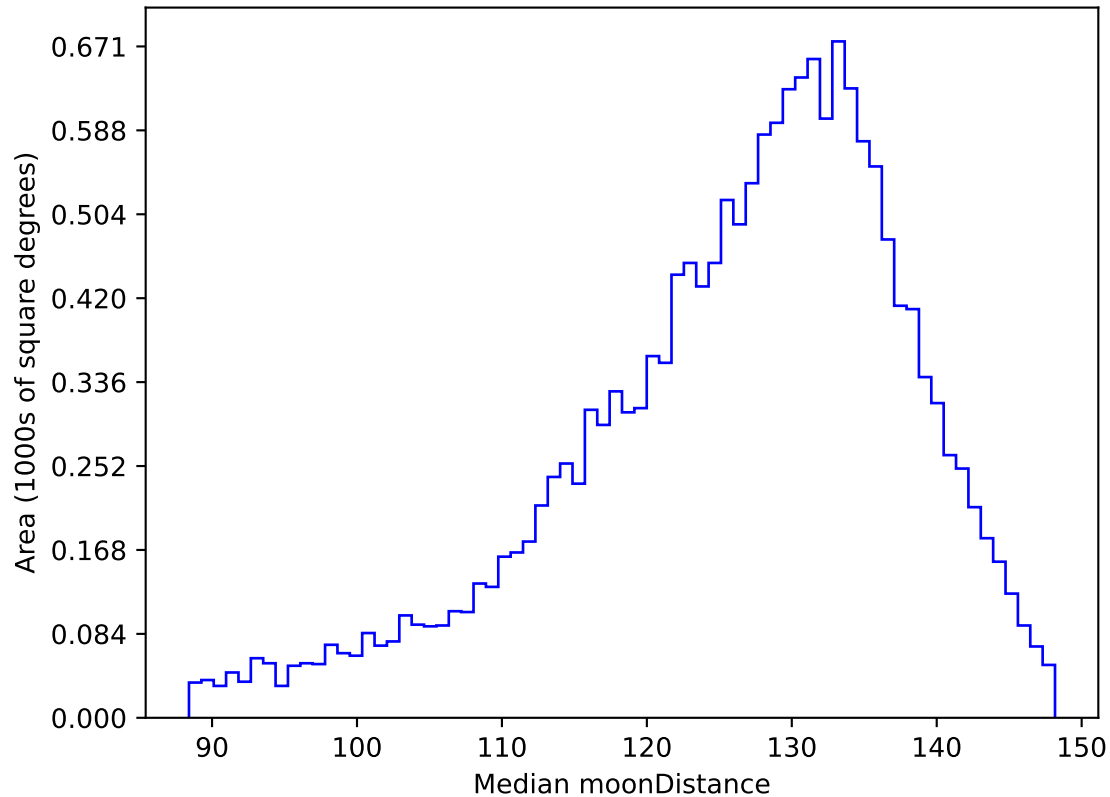
too_elab_heavy_r32_d2_griz_v3.4_10yrs WFD u band: Median moonDistance
