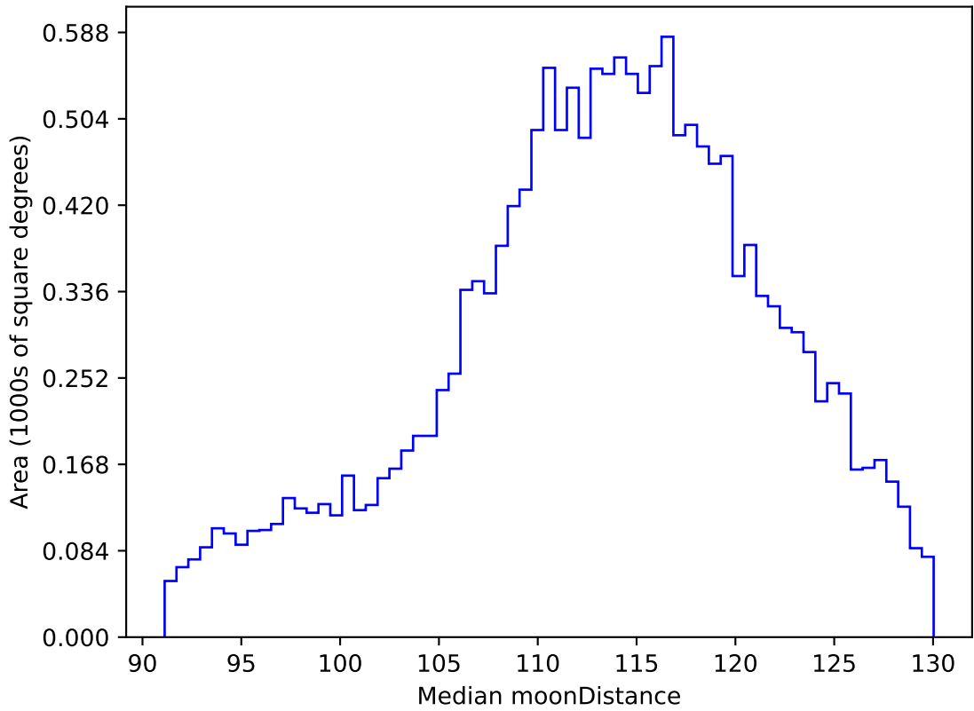
too_elab_heavy_r32_d2_griz_v3.4_10yrs WFD r band: Median moonDistance
