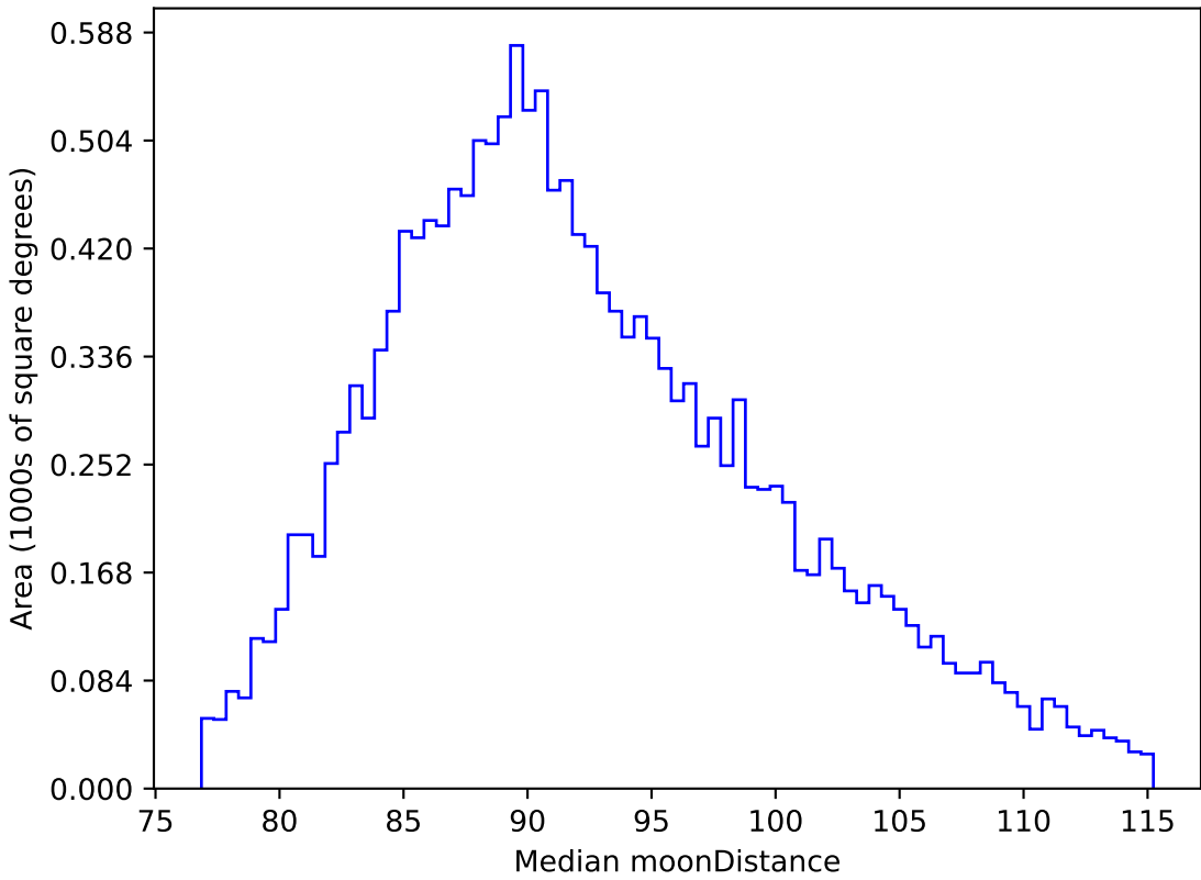
too_elab_heavy_r32_d2_griz_v3.4_10yrs WFD i band: Median moonDistance
