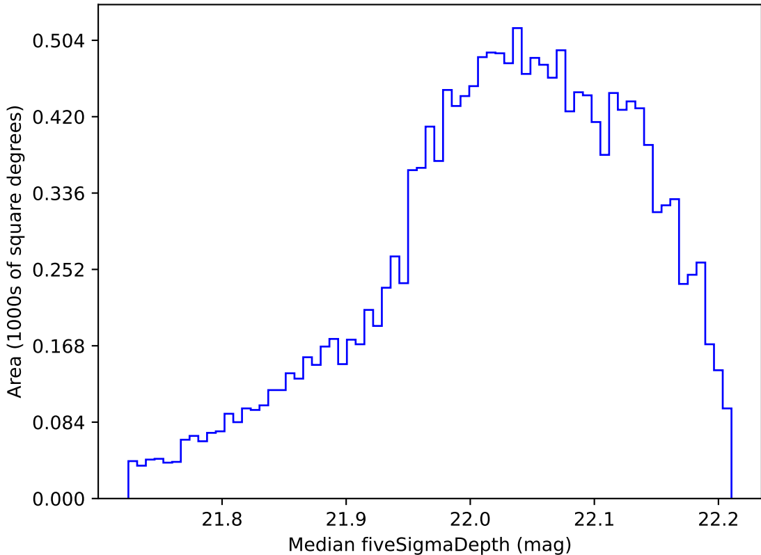
too_elab_heavy_r32_d2_griz_v3.4_10yrs WFD y band: Median fiveSigmaDepth
