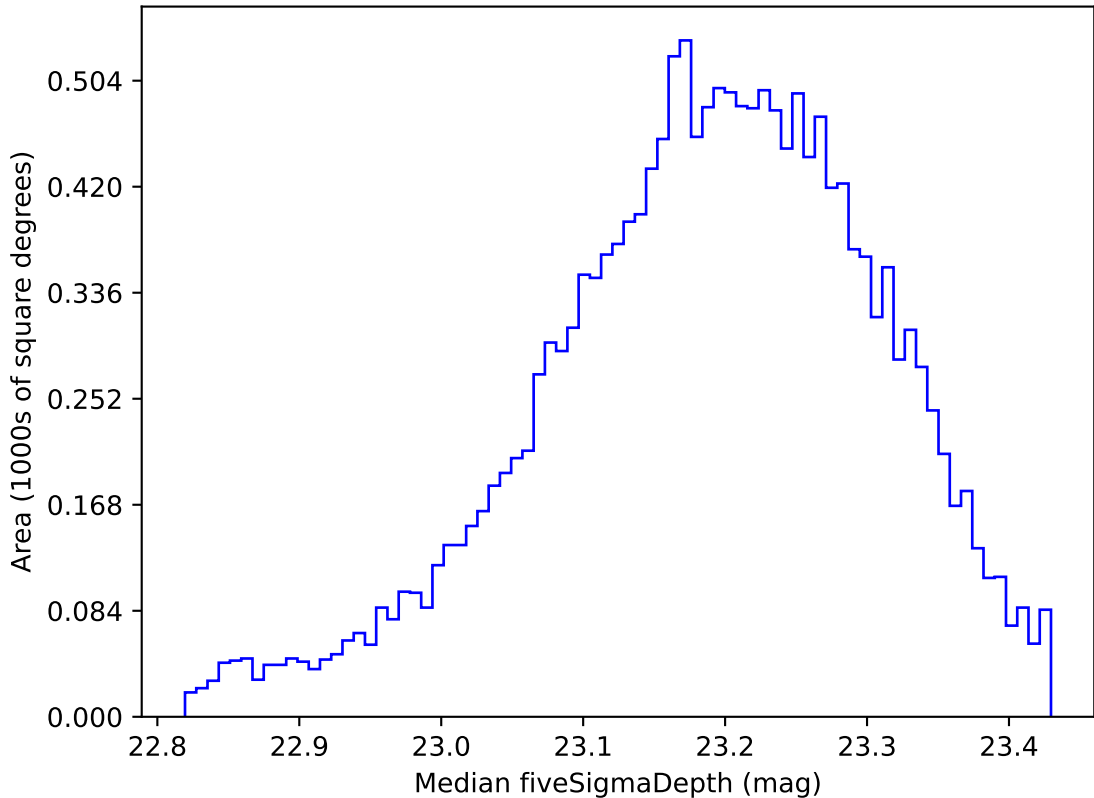
too_elab_heavy_r32_d2_griz_v3.4_10yrs WFD u band: Median fiveSigmaDepth
