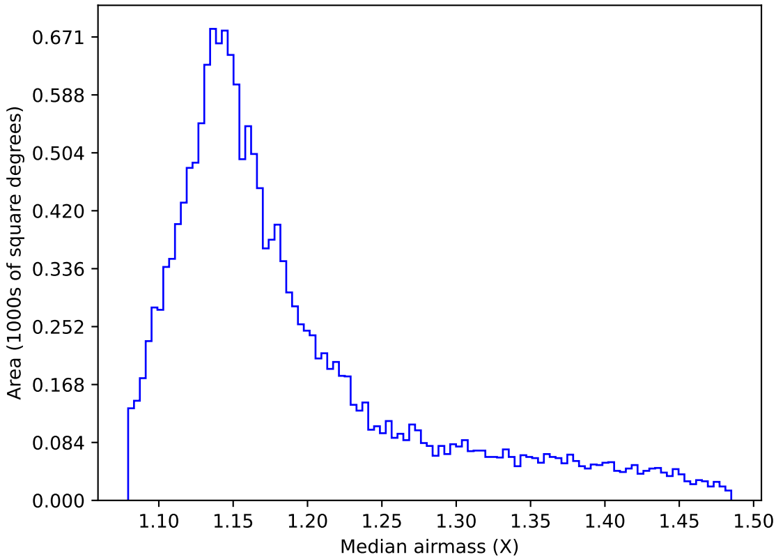
too_elab_heavy_r32_d2_griz_v3.4_10yrs WFD g band: Median airmass
