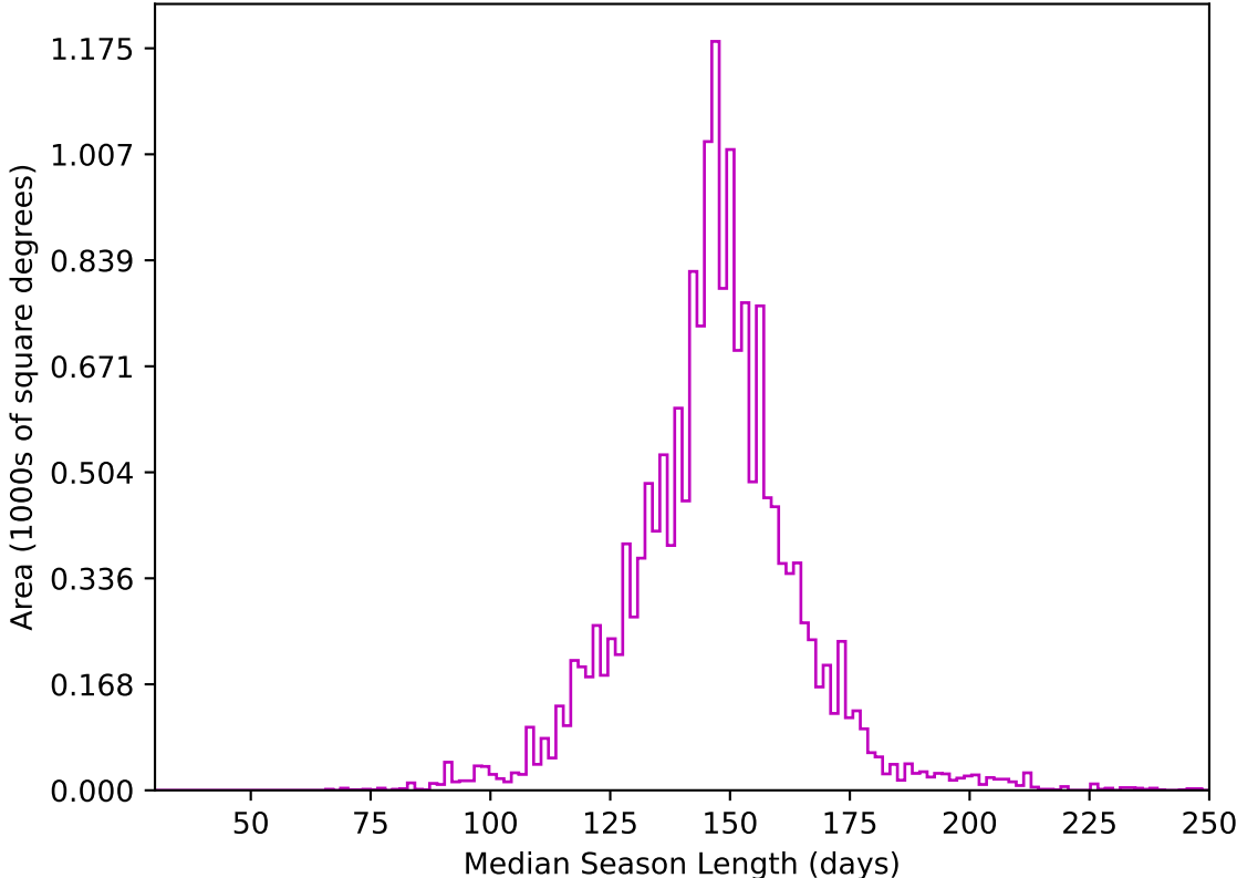
too_elab_heavy_r32_d2_griz_v3.4_10yrs WFD z band: Median Season Length
