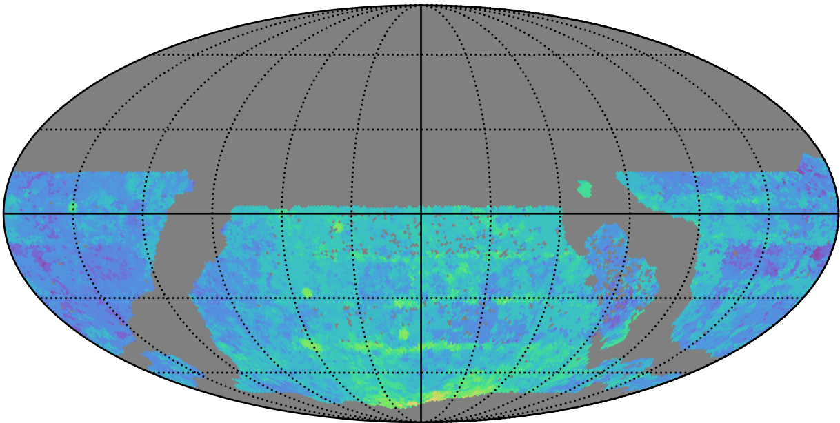
too_elab_heavy_r32_d2_griz_v3.4_10yrs WFD y band: Median Season Length
