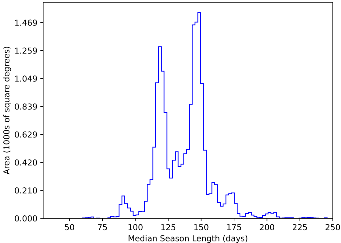
too_elab_heavy_r32_d2_griz_v3.4_10yrs WFD y band: Median Season Length
