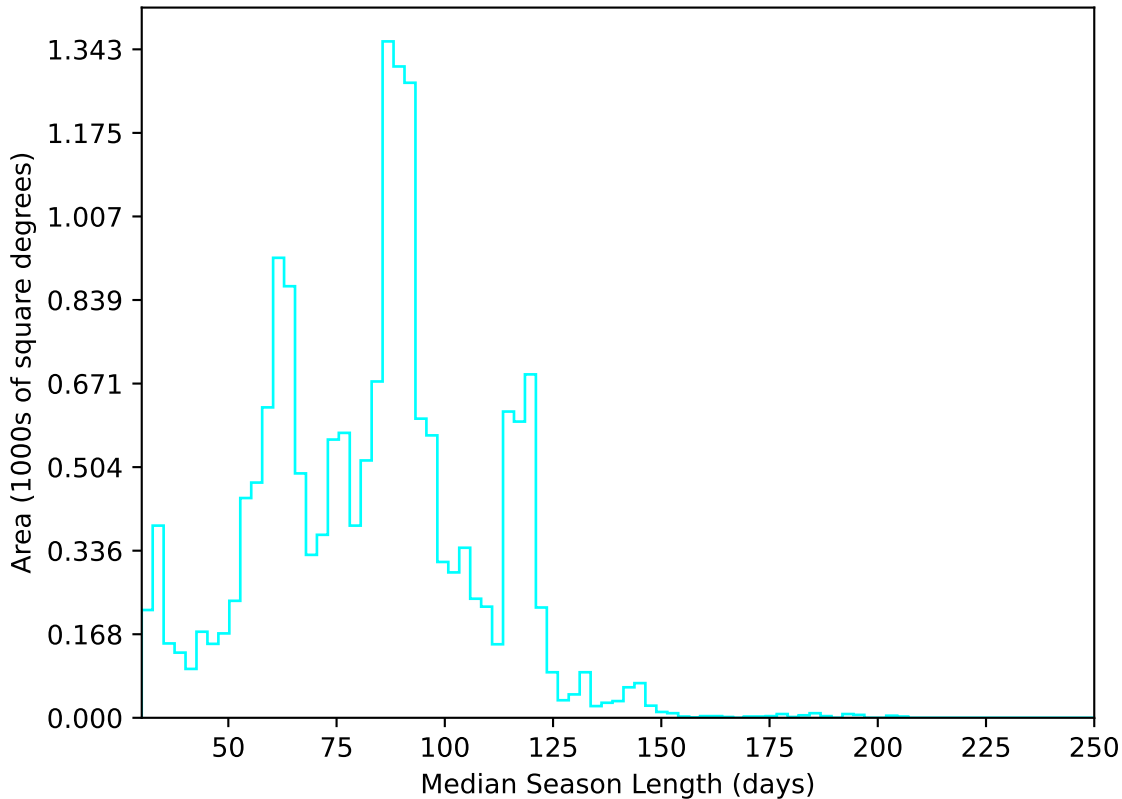
too_elab_heavy_r32_d2_griz_v3.4_10yrs WFD u band: Median Season Length
