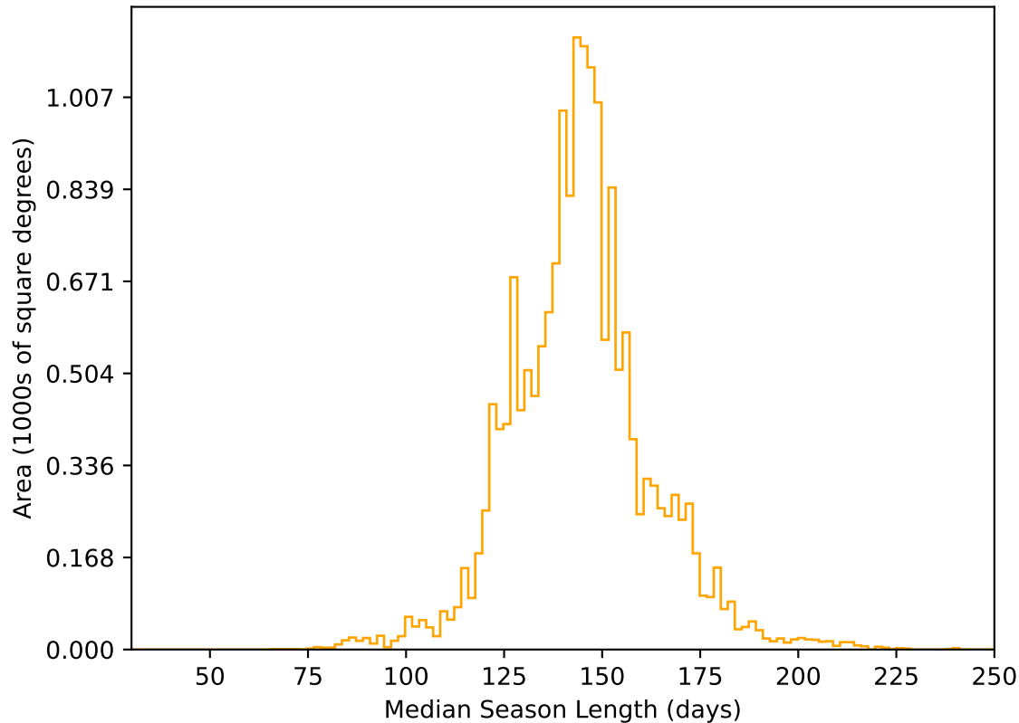
too_elab_heavy_r32_d2_griz_v3.4_10yrs WFD r band: Median Season Length
