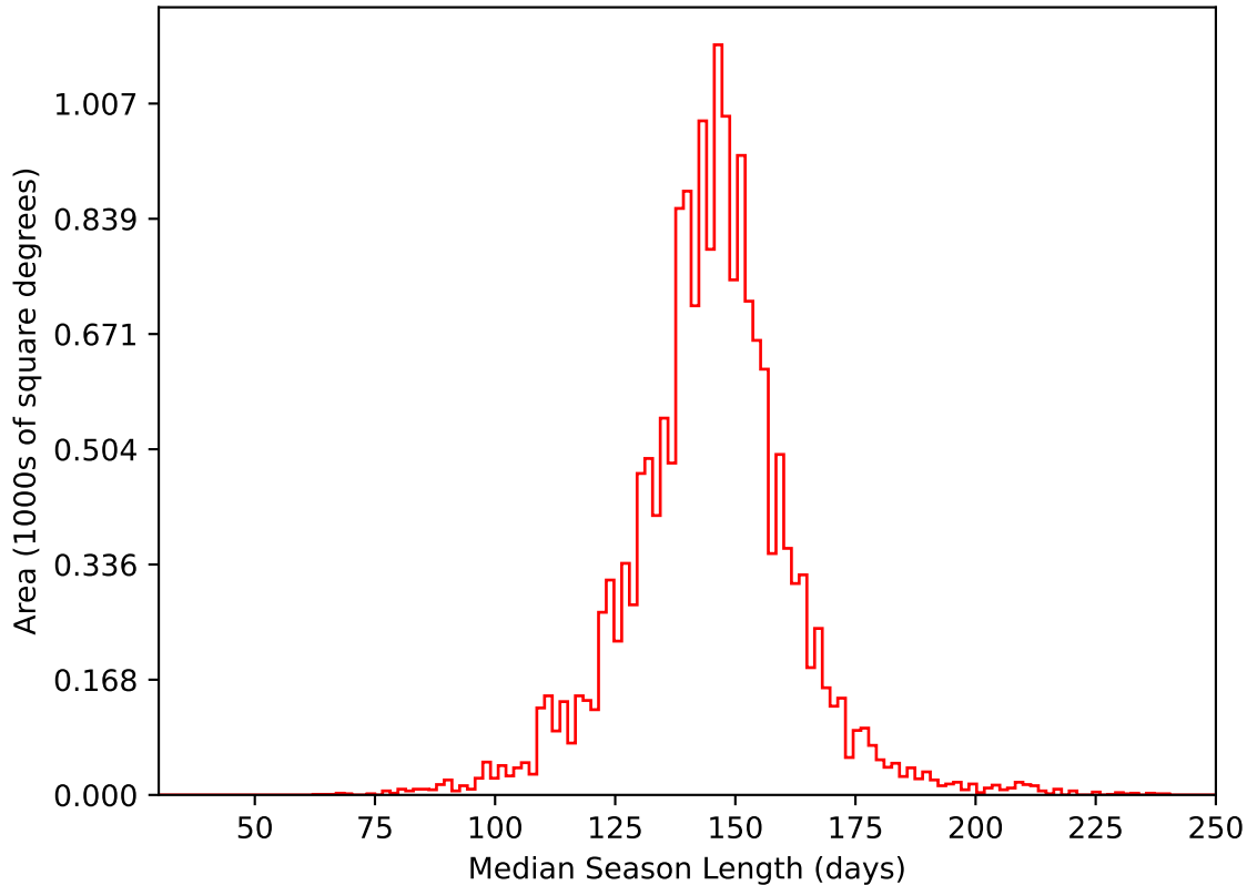
too_elab_heavy_r32_d2_griz_v3.4_10yrs WFD i band: Median Season Length
