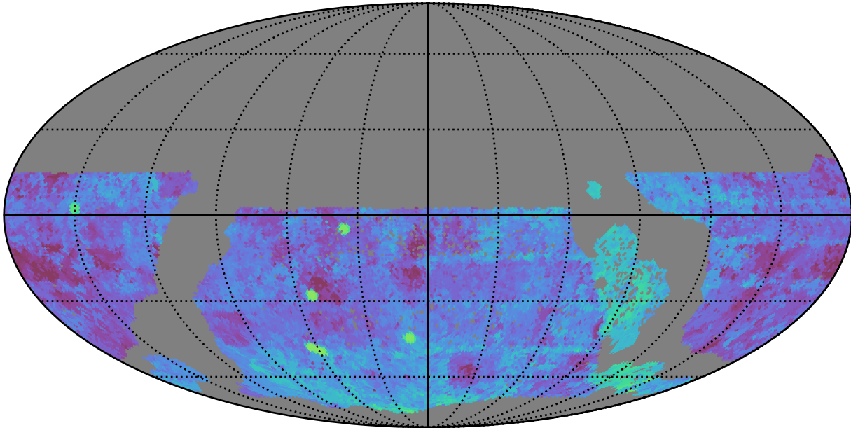
too_elab_heavy_r32_d2_griz_v3.4_10yrs WFD g band: Median Season Length
