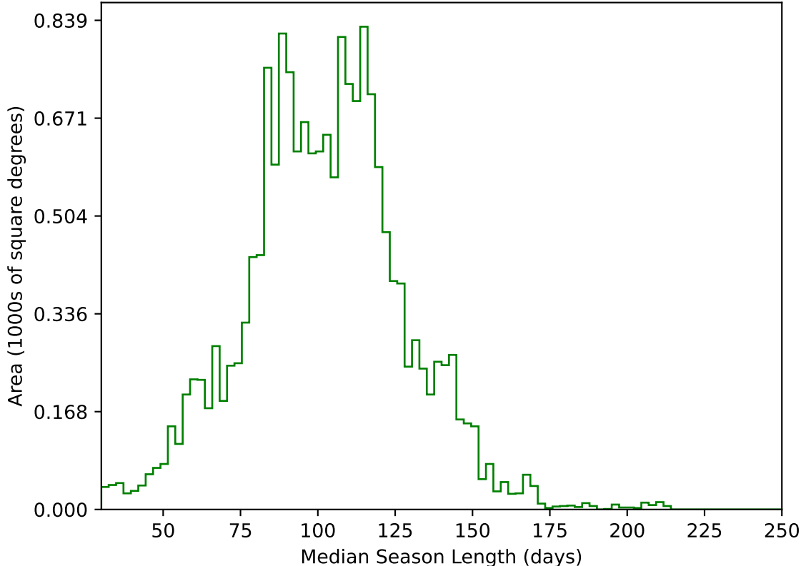
too_elab_heavy_r32_d2_griz_v3.4_10yrs WFD g band: Median Season Length
