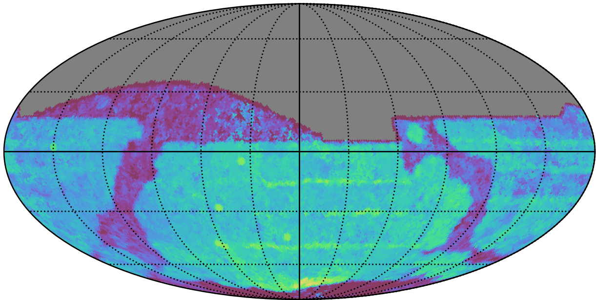
too_elab_heavy_r32_d2_griz_v3.4_10yrs All sky z band: Median Season Length
