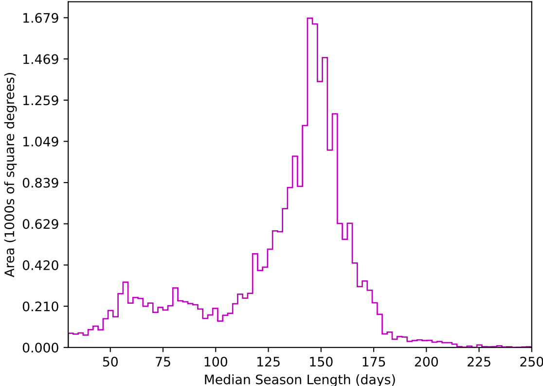
too_elab_heavy_r32_d2_griz_v3.4_10yrs All sky z band: Median Season Length
