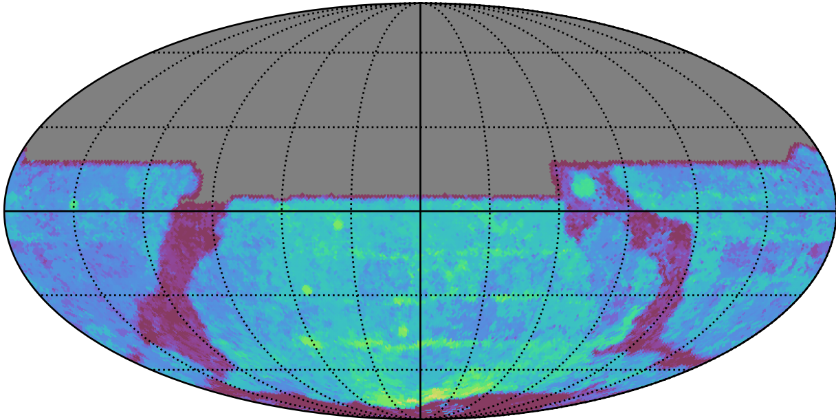
too_elab_heavy_r32_d2_griz_v3.4_10yrs All sky y band: Median Season Length
