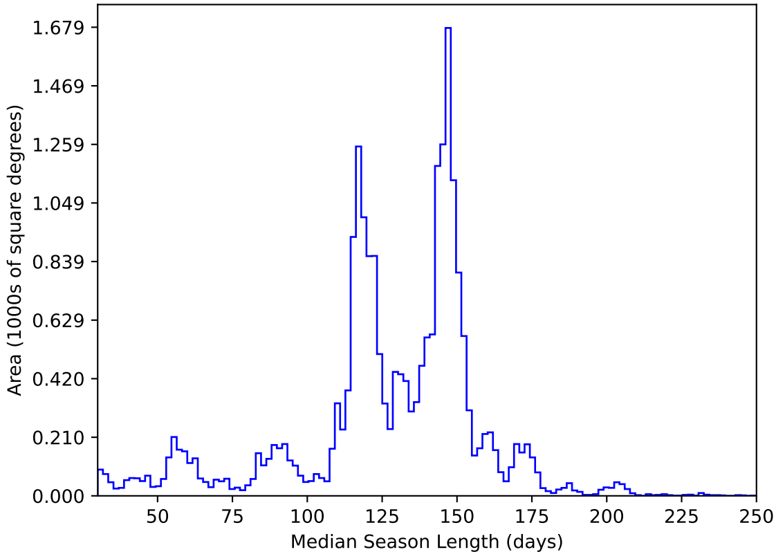
too_elab_heavy_r32_d2_griz_v3.4_10yrs All sky y band: Median Season Length
