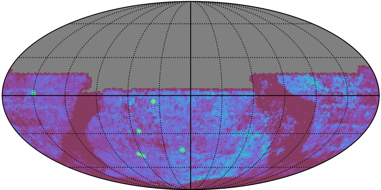
too_elab_heavy_r32_d2_griz_v3.4_10yrs All sky u band: Median Season Length
