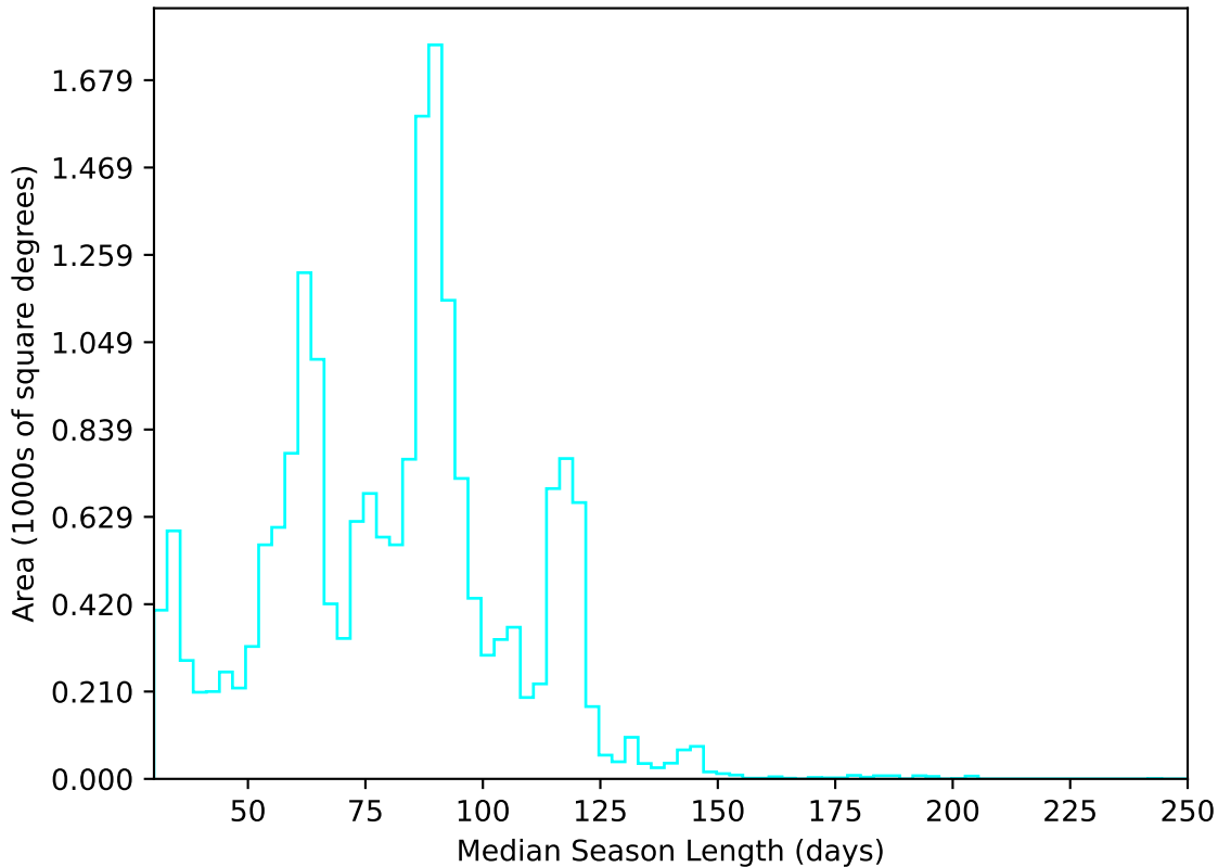
too_elab_heavy_r32_d2_griz_v3.4_10yrs All sky u band: Median Season Length
