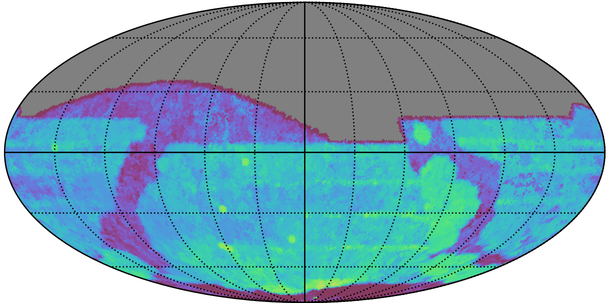
too_elab_heavy_r32_d2_griz_v3.4_10yrs All sky r band: Median Season Length
