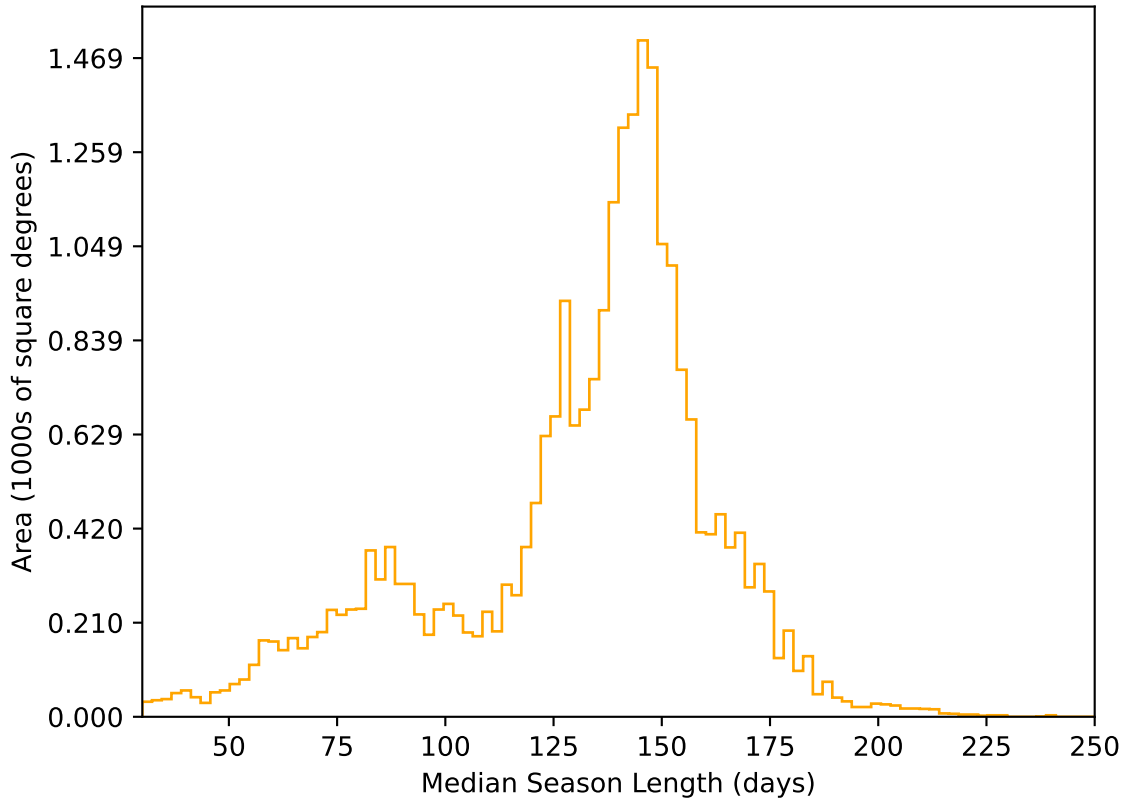
too_elab_heavy_r32_d2_griz_v3.4_10yrs All sky r band: Median Season Length
