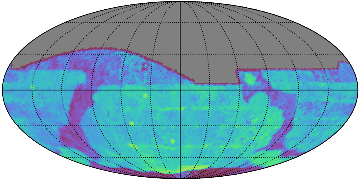
too_elab_heavy_r32_d2_griz_v3.4_10yrs All sky i band: Median Season Length
