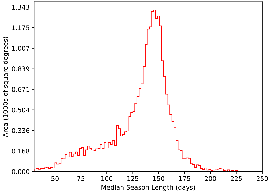
too_elab_heavy_r32_d2_griz_v3.4_10yrs All sky i band: Median Season Length
