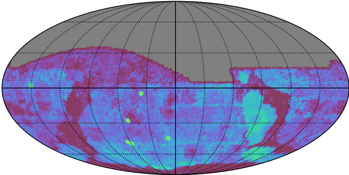
too_elab_heavy_r32_d2_griz_v3.4_10yrs All sky g band: Median Season Length
