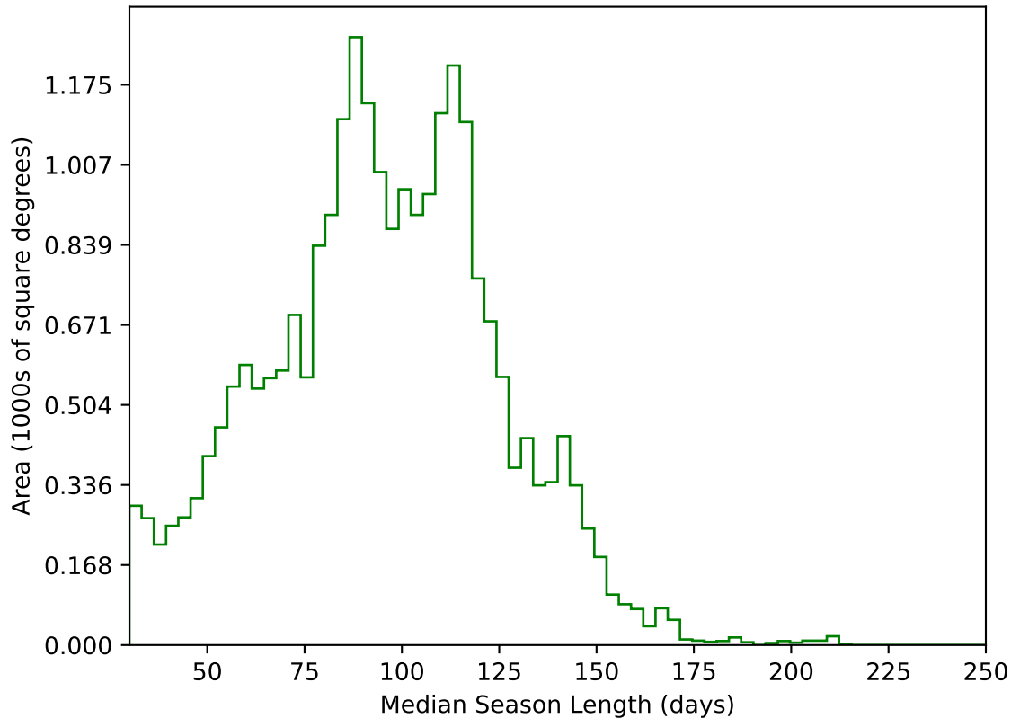
too_elab_heavy_r32_d2_griz_v3.4_10yrs All sky g band: Median Season Length
