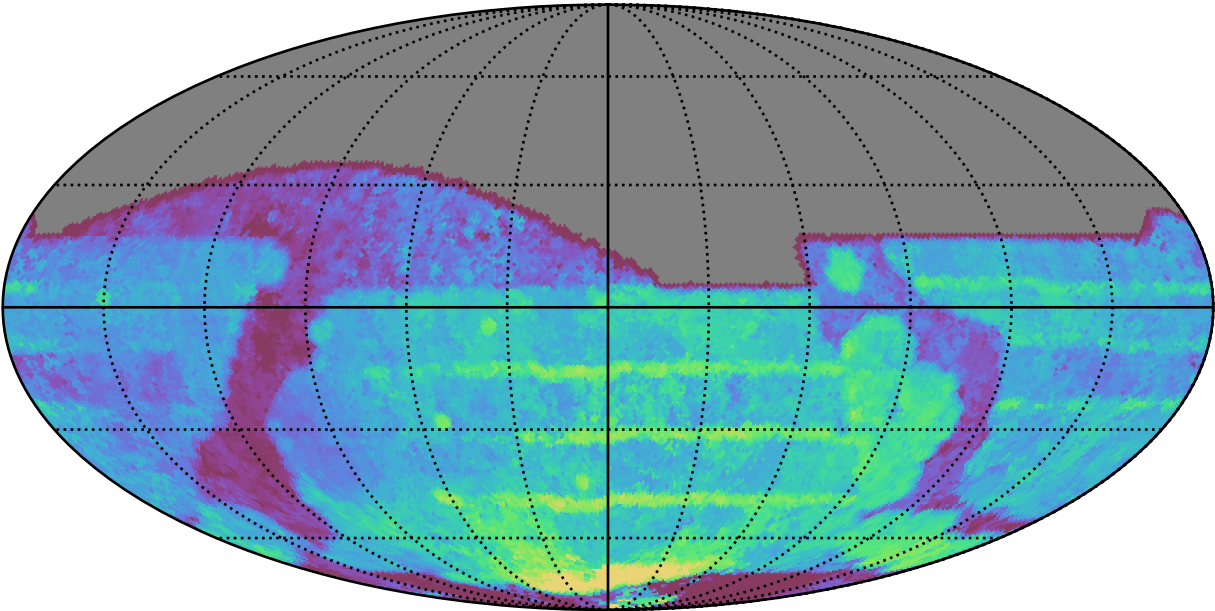
too_elab_heavy_r32_d2_griz_v3.4_10yrs All sky all bands: Median Season Length
